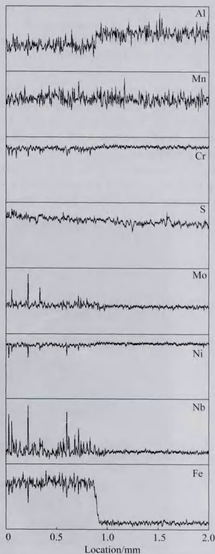
Fig. 4 EPMA-WDS line scan curves across weld fusion line
